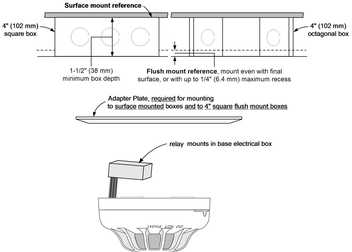
Figure 5: Mounting Information
